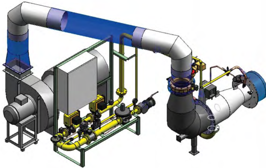
KINEDIZER® LE burner with pipe train, control panel and combustion air blower
