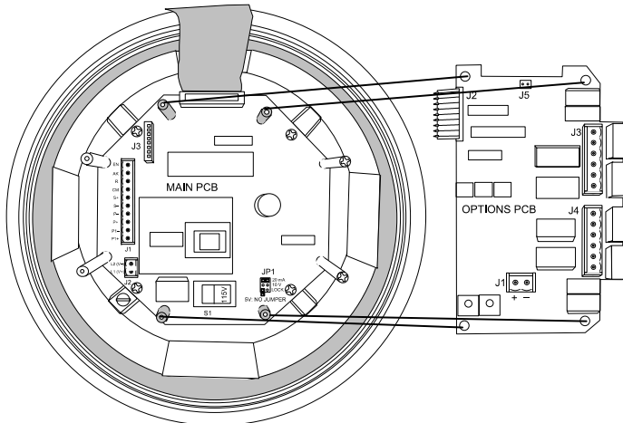
Figure 34. Options Board Installation
